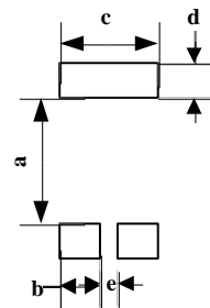
Recommended Land Pattern (Typ.)
